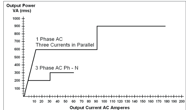
Figure 4: Current output power curve
